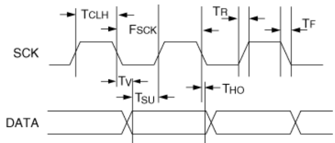
Figure 9 Timing Diagram
